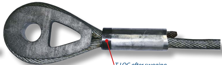
T-LOC after swaging
