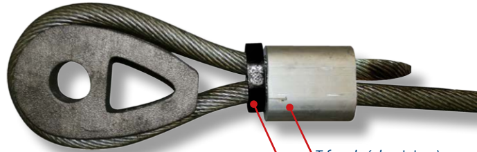
T-ferrule (aluminium) T-LOC before swaging
